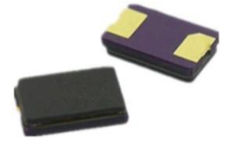
L6.0*W3.5*H1.5mm
